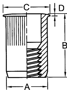
SMALL FLANGE
