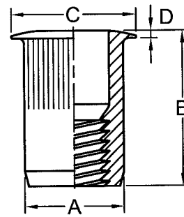
LARGE FLANGE
